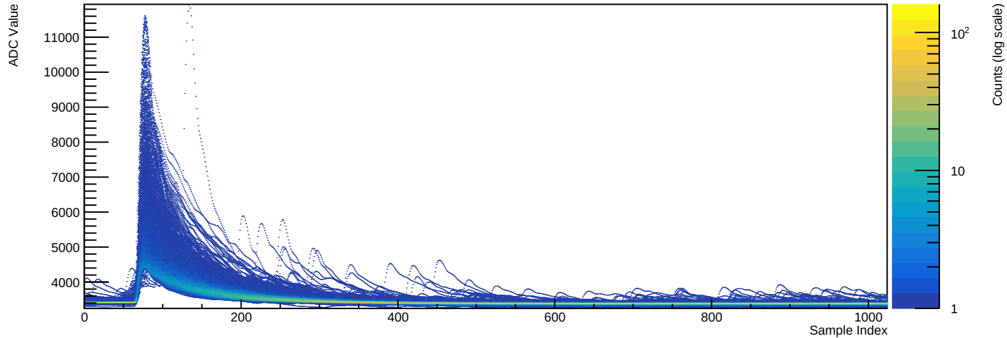
Run 039512 - Channel 2071 (n=2647 waveforms)
