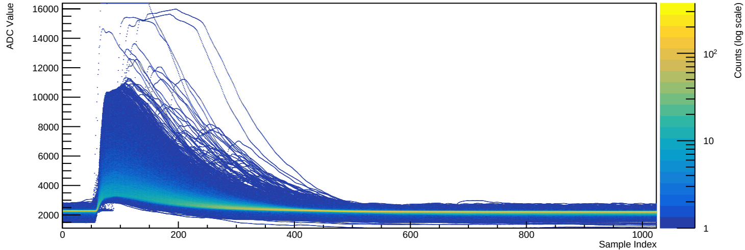
Run 039512 - Channel 2080 (n=14522 waveforms)
