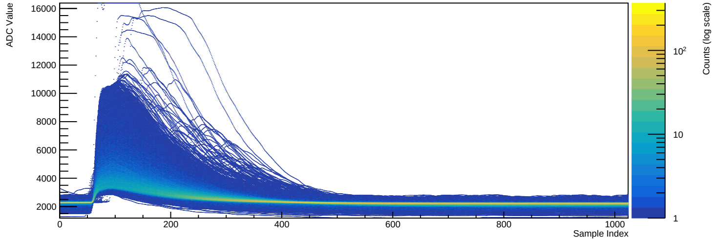
Run 039512 - Channel 2081 (n=14190 waveforms)
