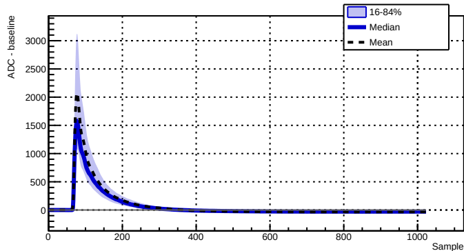
Run 039500 - Channel 2070 - 1189 waveforms
