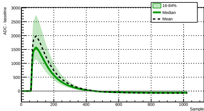
Run 039500 - Channel 2080 - 7761 waveforms
