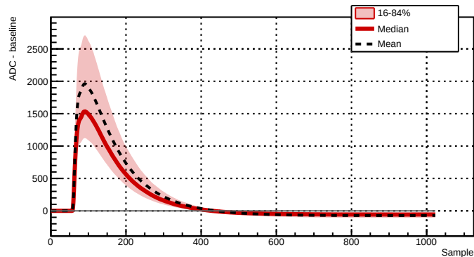
Run 039500 - Channel 2081 - 7437 waveforms
