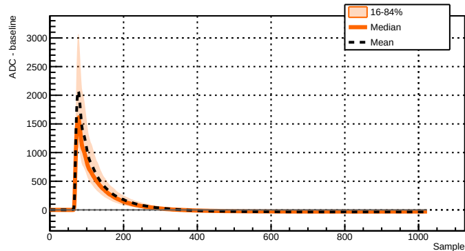
Run 039500 - Channel 2071 - 1129 waveforms
