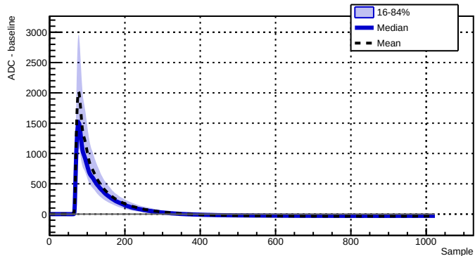
Run 039503 - Channel 2070 - 1548 waveforms
