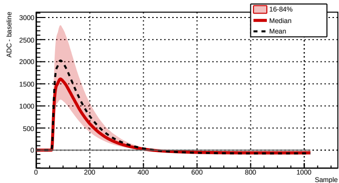
Run 039503 - Channel 2081 - 9338 waveforms
