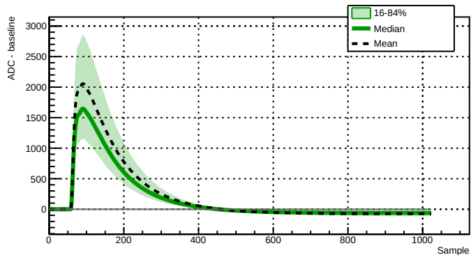
Run 039503 - Channel 2080 - 9674 waveforms
