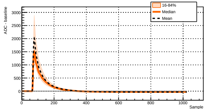
Run 039503 - Channel 2071 - 1462 waveforms
