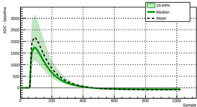
Run 039506 - Channel 2080 - 11696 waveforms
