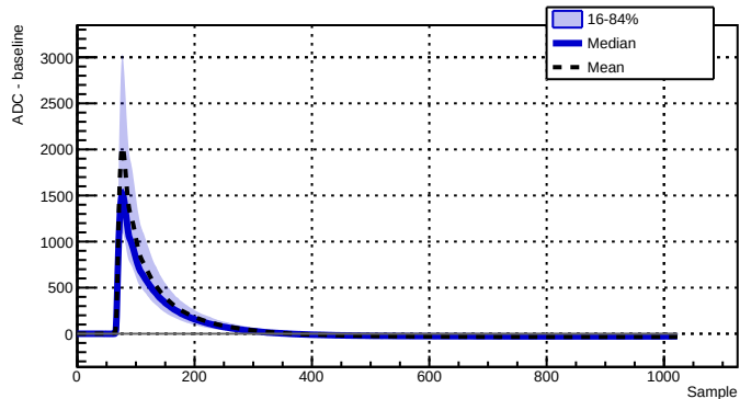
Run 039506 - Channel 2070 - 1947 waveforms
