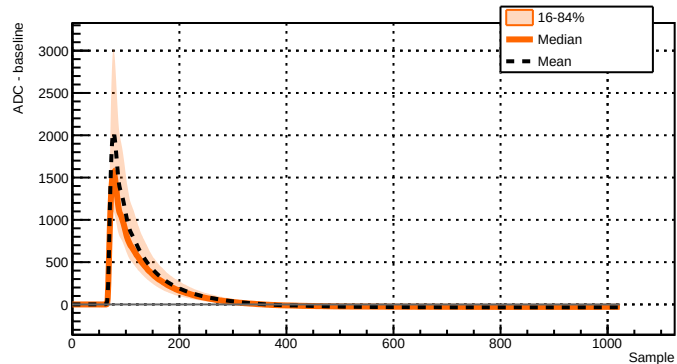
Run 039506 - Channel 2071 - 1818 waveforms
