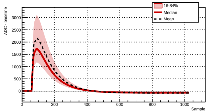
Run 039506 - Channel 2081 - 11267 waveforms
