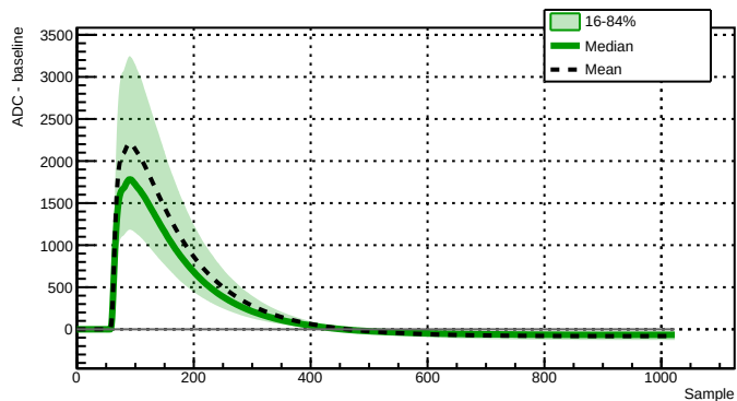
Run 039516 - Channel 2080 - 11876 waveforms
