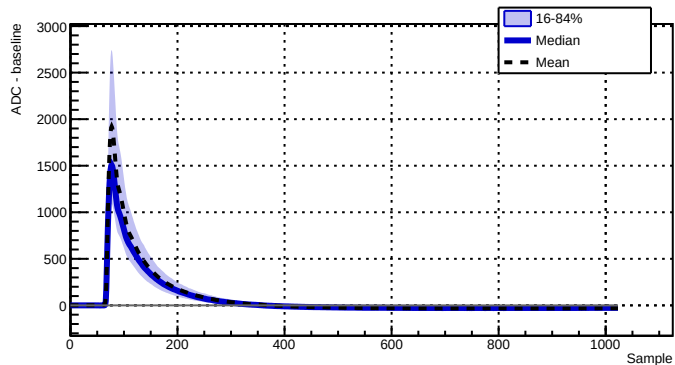
Run 039516 - Channel 2070 - 2026 waveforms
