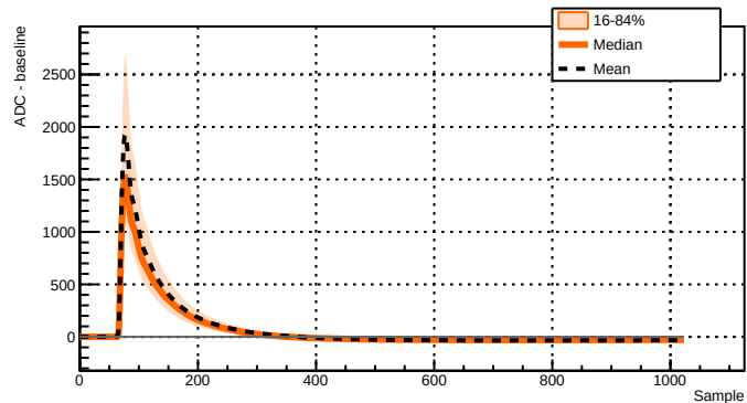
Run 039516 - Channel 2071 - 1940 waveforms
