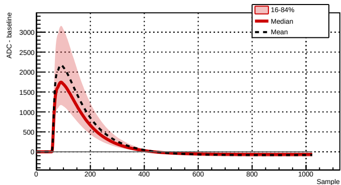
Run 039516 - Channel 2081 - 11579 waveforms
