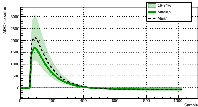
Run 039519 - Channel 2080 - 10652 waveforms
