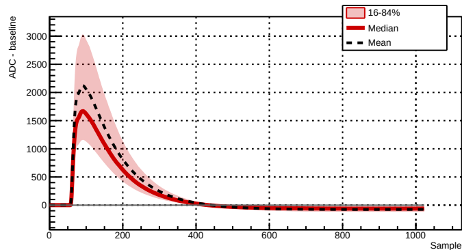
Run 039519 - Channel 2081 - 10242 waveforms
