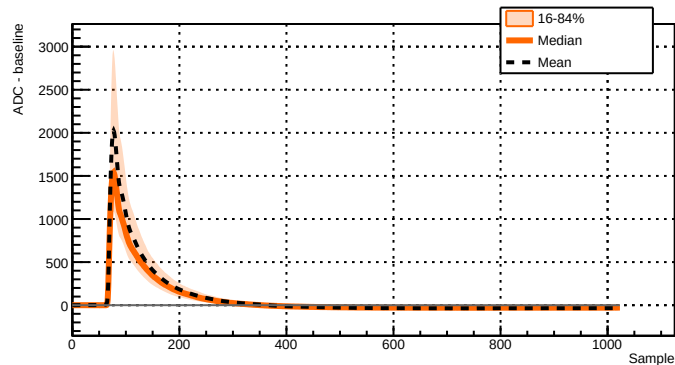
Run 039519 - Channel 2071 - 1598 waveforms
