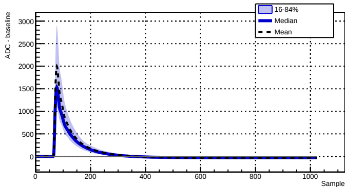
Run 039519 - Channel 2070 - 1701 waveforms
