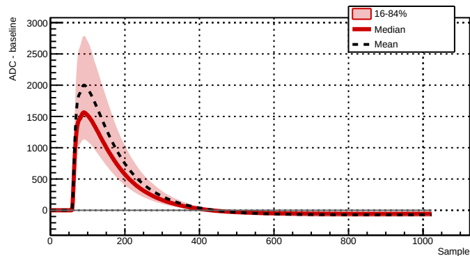
Run 039526 - Channel 2081 - 7949 waveforms
