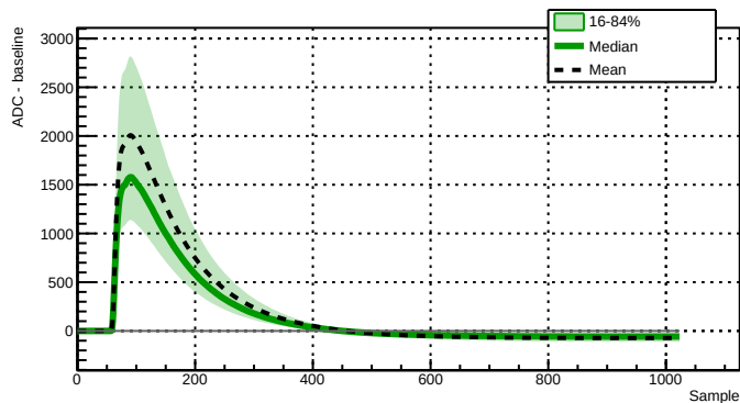
Run 039526 - Channel 2080 - 8352 waveforms
