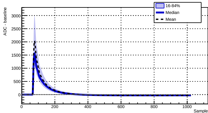
Run 039526 - Channel 2070 - 1304 waveforms
