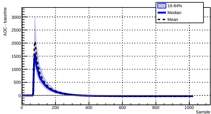
Run 039528 - Channel 2070 - 1194 waveforms
