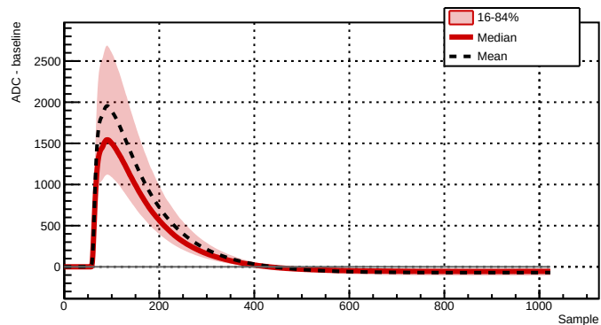
Run 039528 - Channel 2081 - 7605 waveforms
