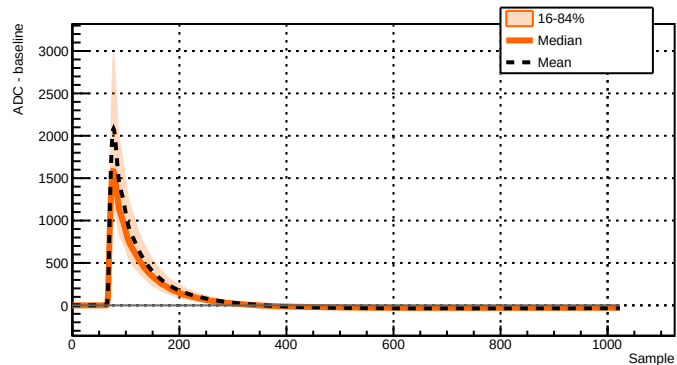
Run 039528 - Channel 2071 - 1101 waveforms
