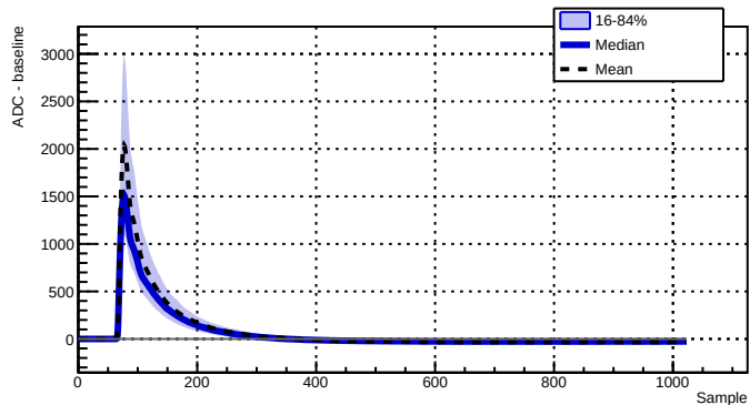
Run 039529 - Channel 2070 - 1169 waveforms
