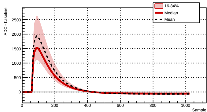
Run 039529 - Channel 2081 - 7411 waveforms
