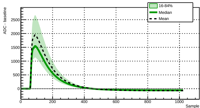
Run 039529 - Channel 2080 - 7742 waveforms
