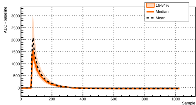
Run 039529 - Channel 2071 - 1091 waveforms
