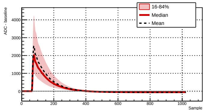
Run 039502 - Channel 2061 - 8593 waveforms
