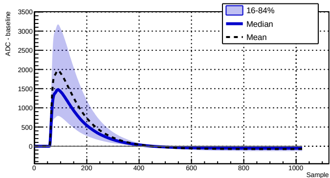
Run 039502 - Channel 2050 - 18420 waveforms
