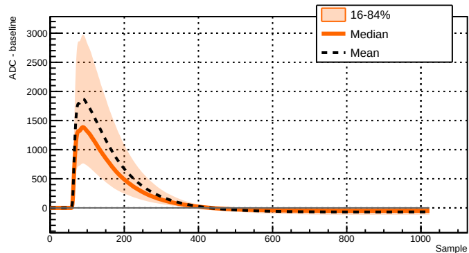
Run 039502 - Channel 2051 - 11798 waveforms
