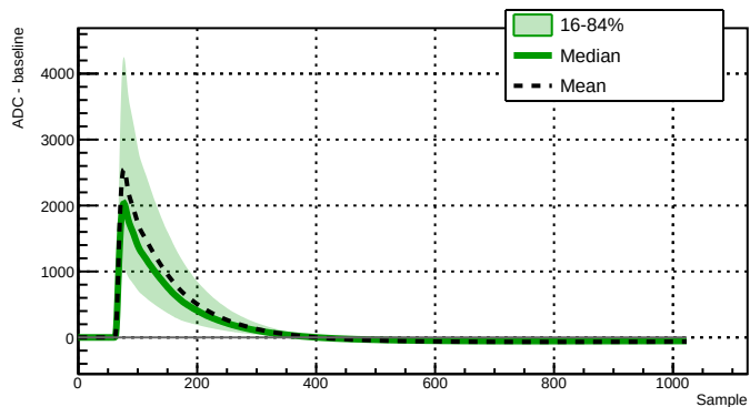
Run 039502 - Channel 2060 - 13339 waveforms
