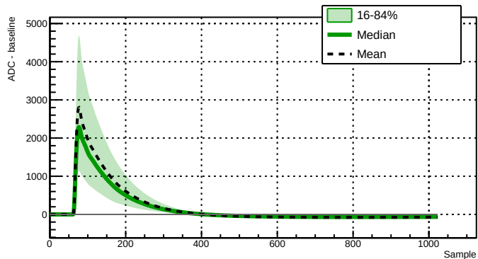
Run 039507 - Channel 2060 - 16392 waveforms
