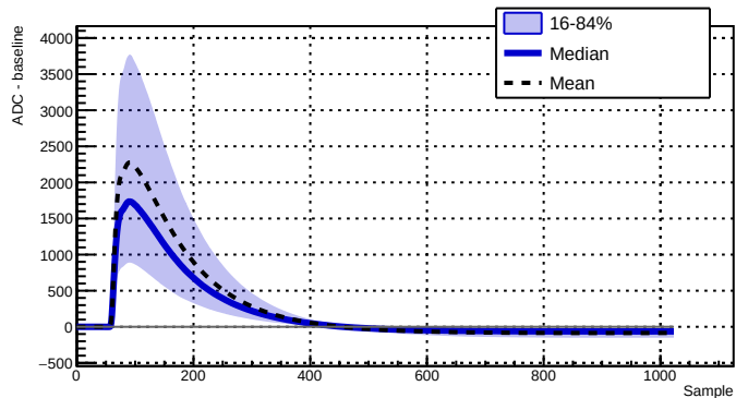
Run 039507 - Channel 2050 - 22387 waveforms
