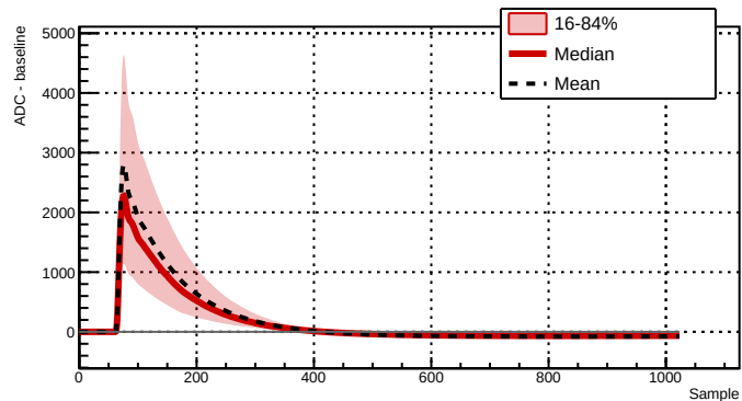
Run 039507 - Channel 2061 - 10910 waveforms
