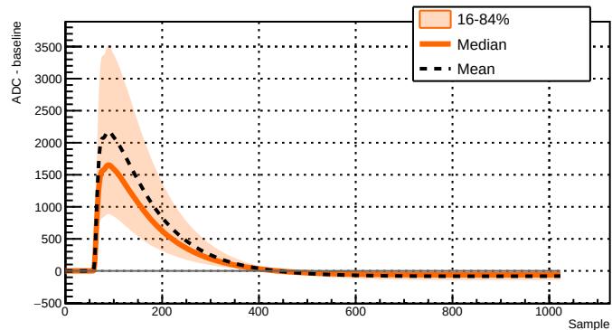
Run 039507 - Channel 2051 - 14844 waveforms
