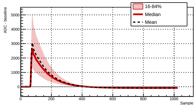
Run 039510 - Channel 2061 - 10888 waveforms
