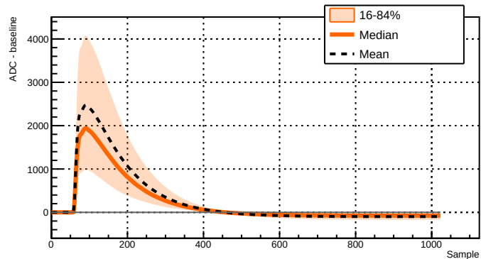
Run 039510 - Channel 2051 - 16354 waveforms
