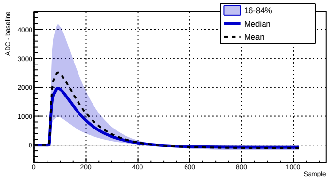
Run 039510 - Channel 2050 - 23664 waveforms
