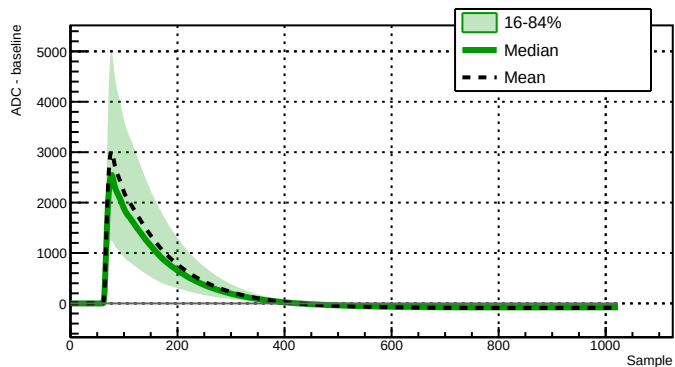
Run 039510 - Channel 2060 - 16912 waveforms
