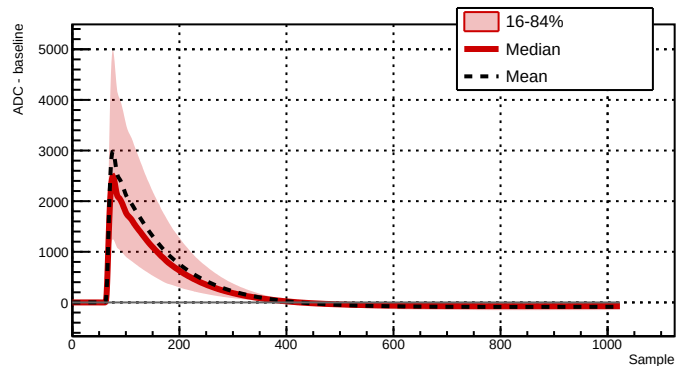
Run 039511 - Channel 2061 - 11263 waveforms
