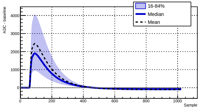
Run 039511 - Channel 2050 - 24031 waveforms
