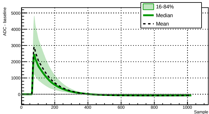
Run 039511 - Channel 2060 - 17347 waveforms
