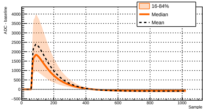
Run 039511 - Channel 2051 - 16426 waveforms
