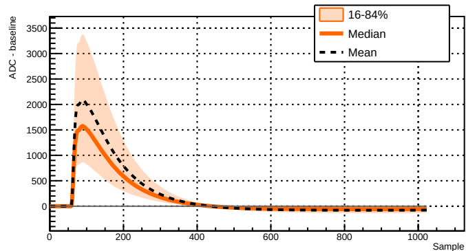
Run 039516 - Channel 2051 - 13909 waveforms
