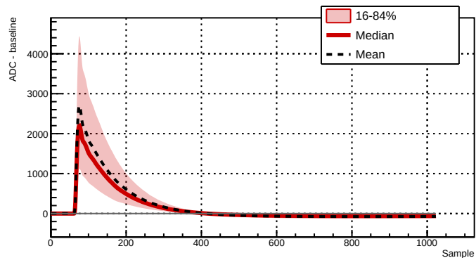
Run 039516 - Channel 2061 - 10053 waveforms
