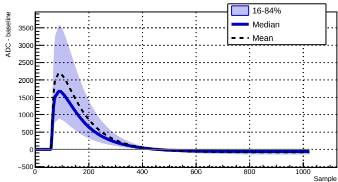
Run 039516 - Channel 2050 - 20929 waveforms
