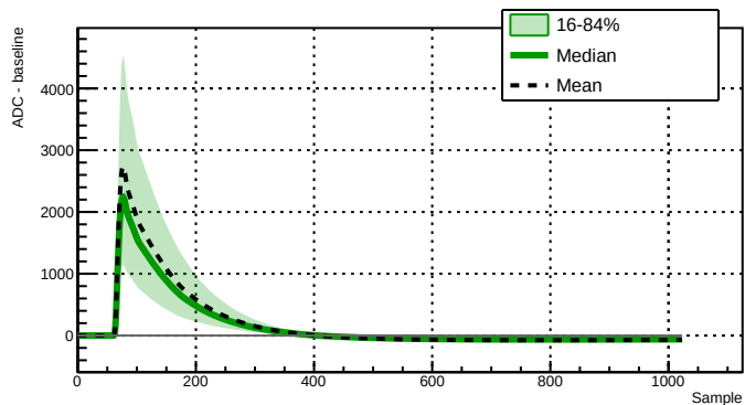
Run 039516 - Channel 2060 - 15086 waveforms
