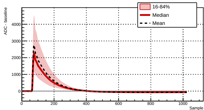
Run 039517 - Channel 2061 - 10055 waveforms
