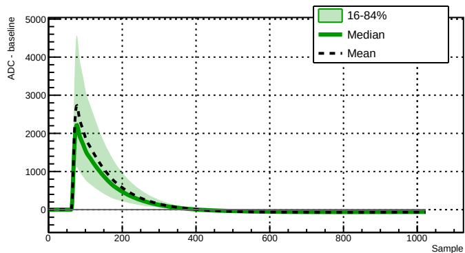
Run 039517 - Channel 2060 - 15310 waveforms
