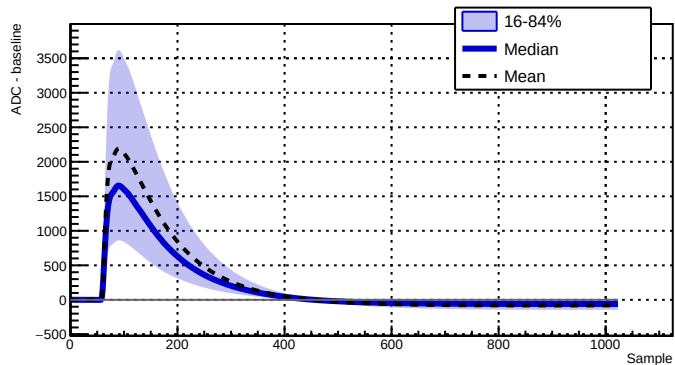
Run 039517 - Channel 2050 - 20742 waveforms
