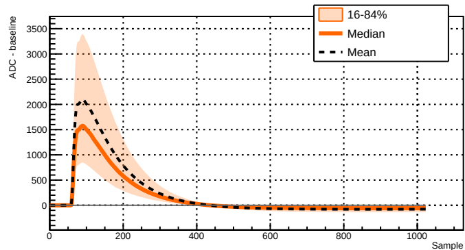
Run 039517 - Channel 2051 - 13778 waveforms
