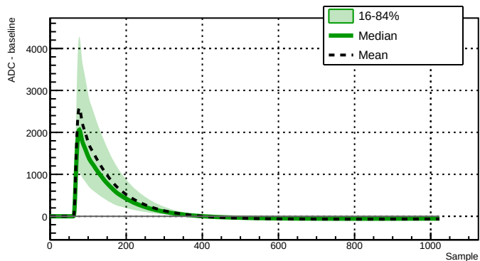
Run 039522 - Channel 2060 - 13560 waveforms
