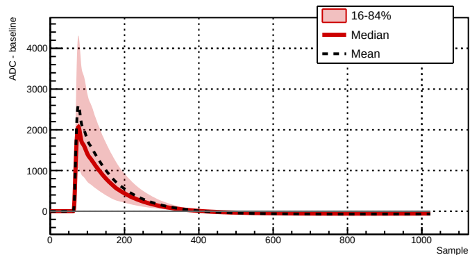
Run 039522 - Channel 2061 - 8924 waveforms
