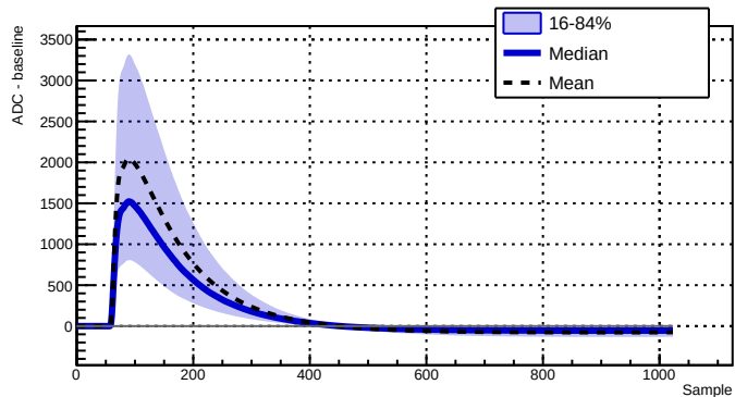
Run 039522 - Channel 2050 - 18611 waveforms
