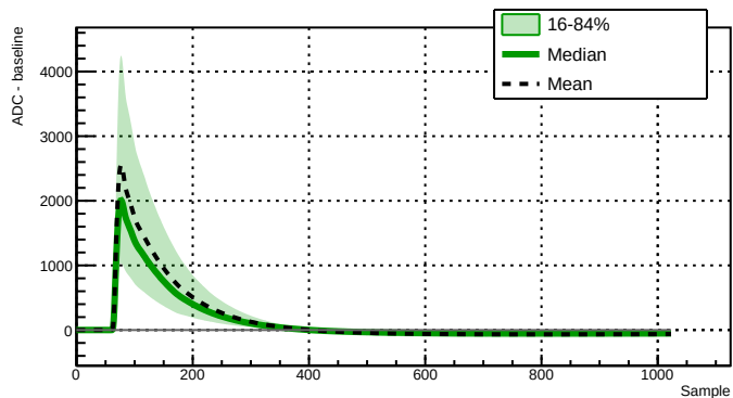
Run 039525 - Channel 2060 - 13080 waveforms
