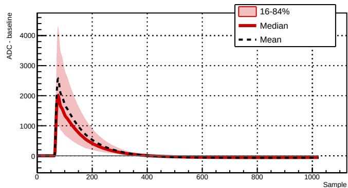
Run 039525 - Channel 2061 - 8490 waveforms
