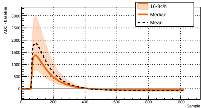
Run 039525 - Channel 2051 - 11423 waveforms
