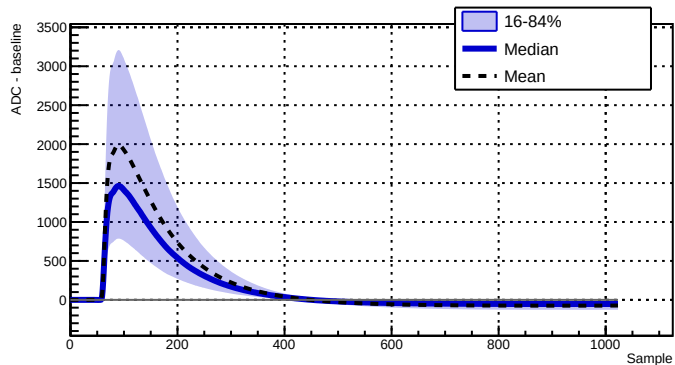
Run 039525 - Channel 2050 - 17897 waveforms
