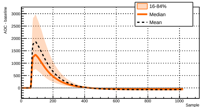
Run 039527 - Channel 2051 - 10865 waveforms
