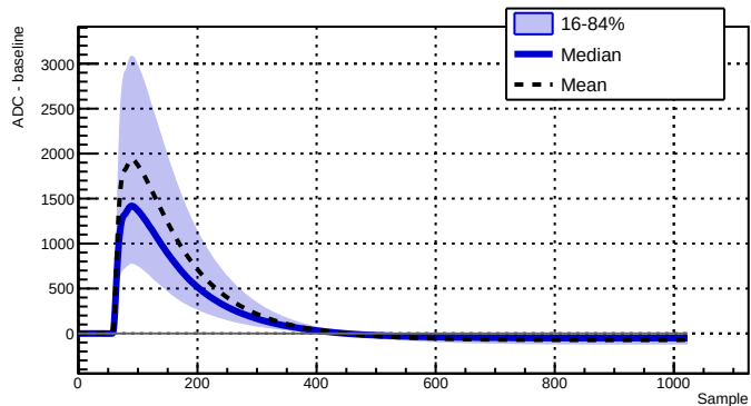
Run 039527 - Channel 2050 - 17314 waveforms
