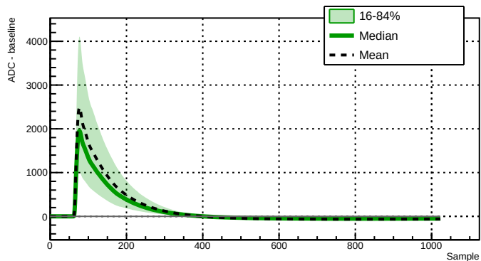
Run 039527 - Channel 2060 - 12595 waveforms
