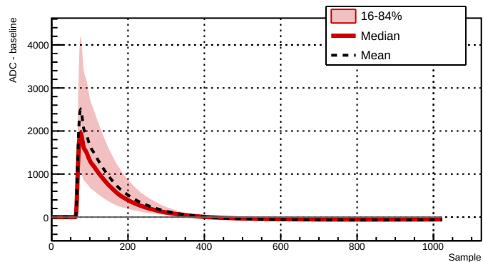
Run 039527 - Channel 2061 - 8083 waveforms
