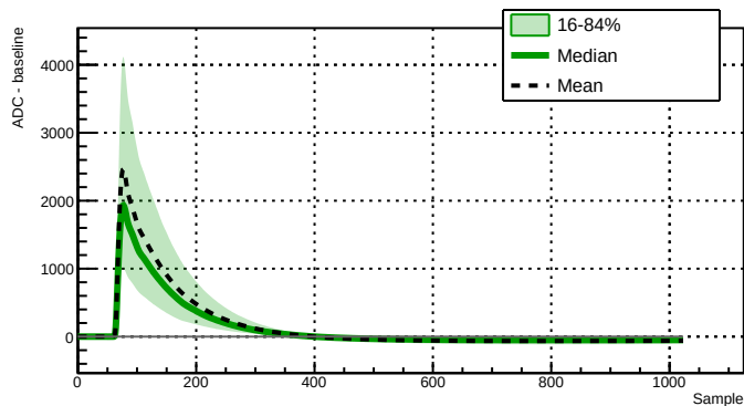
Run 039528 - Channel 2060 - 12498 waveforms
