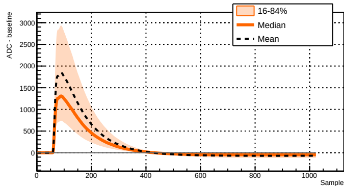
Run 039528 - Channel 2051 - 10587 waveforms
