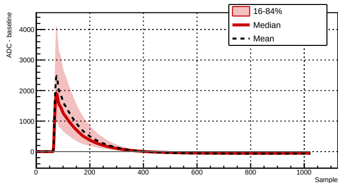
Run 039528 - Channel 2061 - 8105 waveforms
