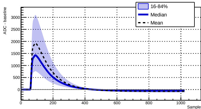
Run 039528 - Channel 2050 - 16996 waveforms
