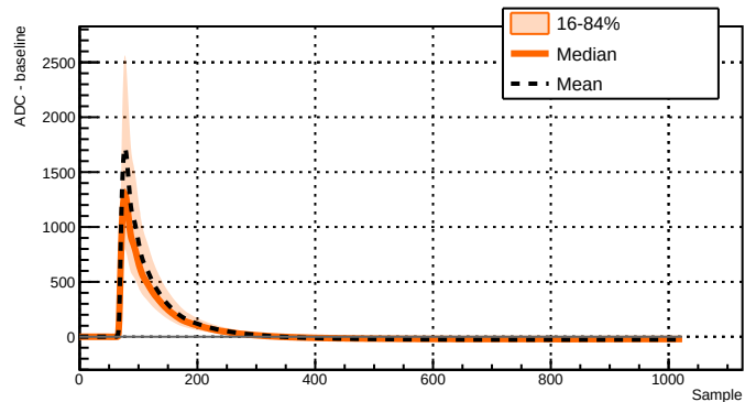
Run 039502 - Channel 2071 - 5285 waveforms
