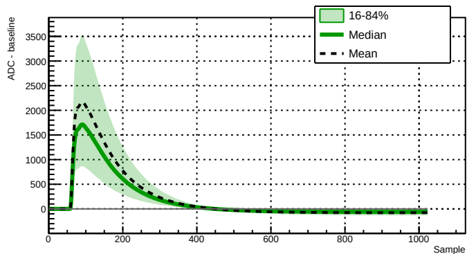
Run 039502 - Channel 2080 - 23003 waveforms
