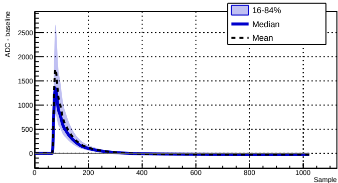
Run 039503 - Channel 2070 - 5281 waveforms
