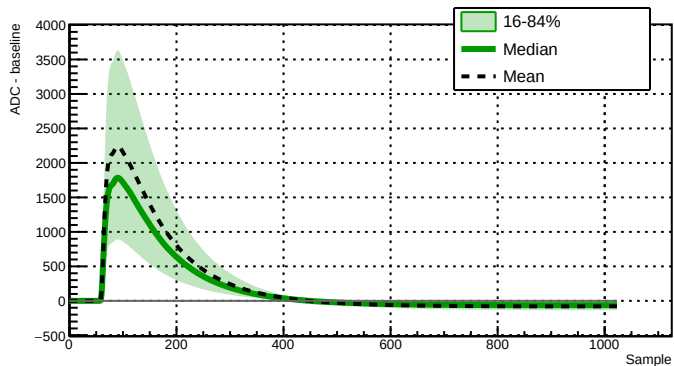
Run 039503 - Channel 2080 - 24271 waveforms
