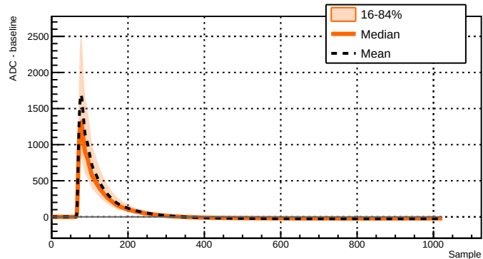
Run 039503 - Channel 2071 - 5512 waveforms
