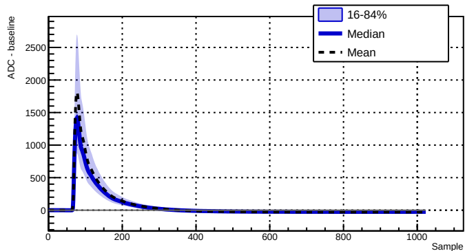
Run 039508 - Channel 2070 - 6390 waveforms
