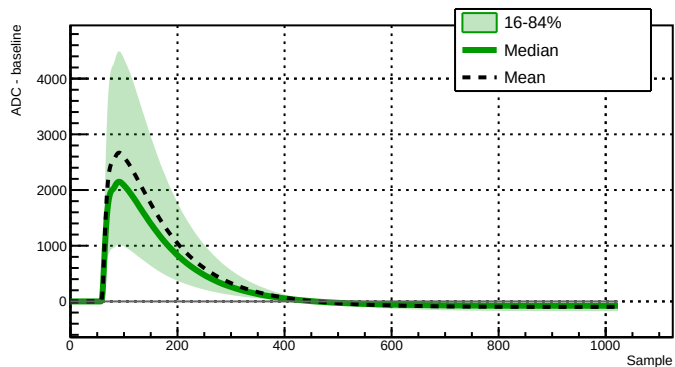
Run 039508 - Channel 2080 - 29125 waveforms
