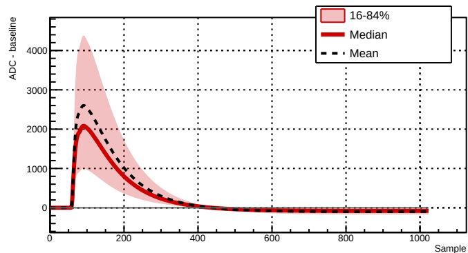
Run 039508 - Channel 2081 - 29448 waveforms
