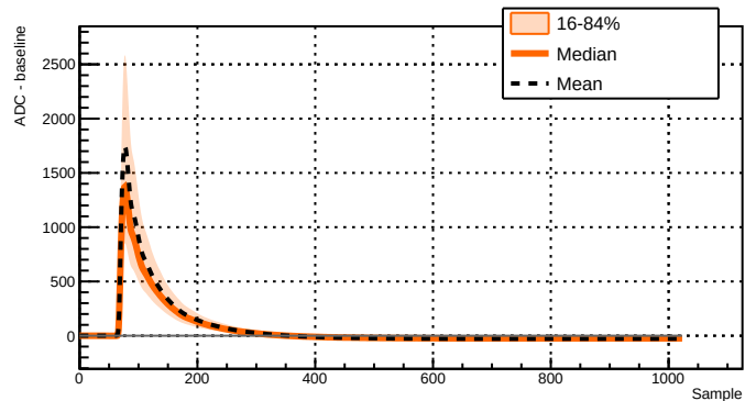
Run 039508 - Channel 2071 - 6855 waveforms
