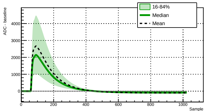
Run 039512 - Channel 2080 - 29100 waveforms
