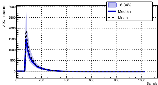
Run 039512 - Channel 2070 - 6453 waveforms
