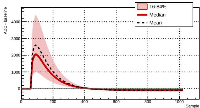
Run 039512 - Channel 2081 - 29612 waveforms
