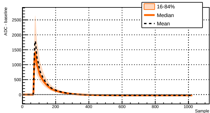
Run 039512 - Channel 2071 - 6923 waveforms
