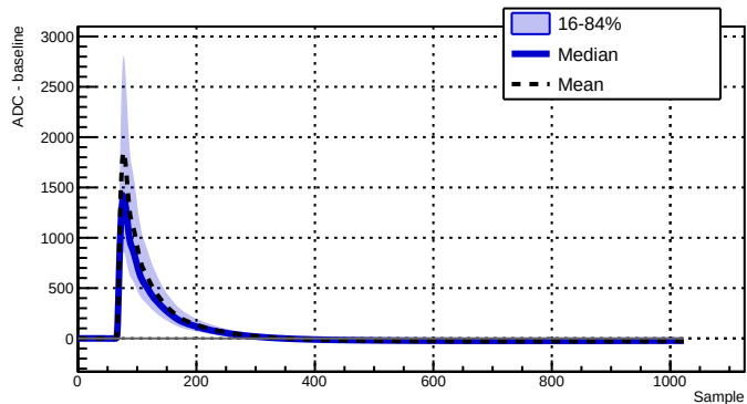
Run 039515 - Channel 2070 - 6054 waveforms
