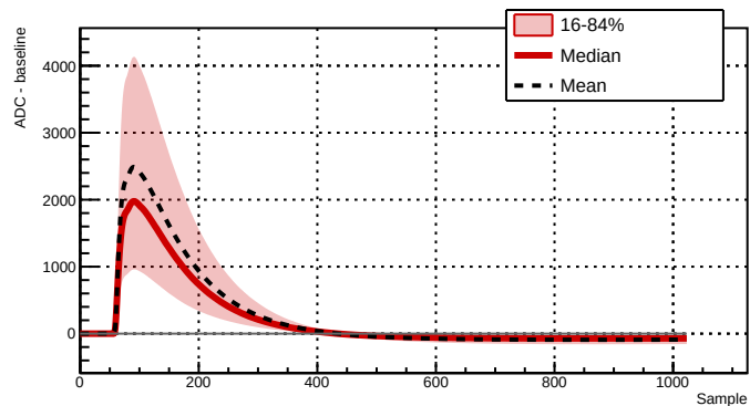
Run 039515 - Channel 2081 - 27274 waveforms
