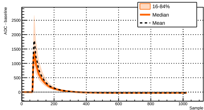
Run 039515 - Channel 2071 - 6330 waveforms
