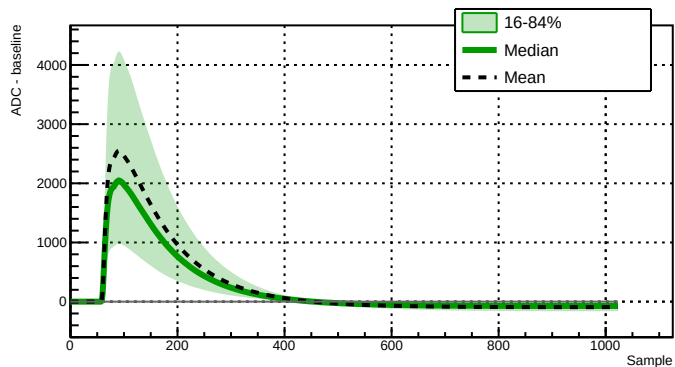
Run 039515 - Channel 2080 - 26799 waveforms
