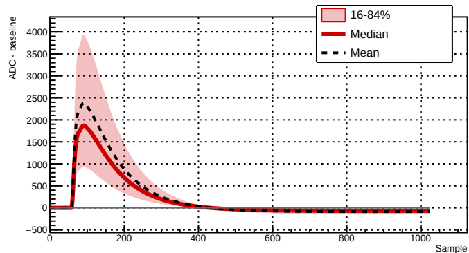
Run 039517 - Channel 2081 - 26704 waveforms
