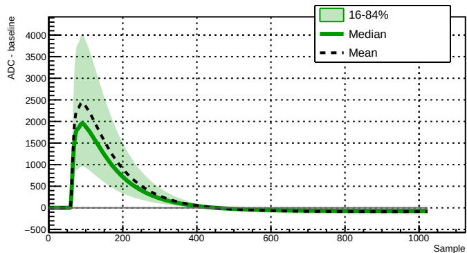
Run 039517 - Channel 2080 - 25961 waveforms
