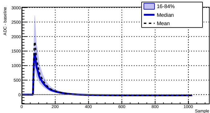
Run 039517 - Channel 2070 - 5651 waveforms
