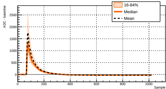
Run 039517 - Channel 2071 - 6010 waveforms
