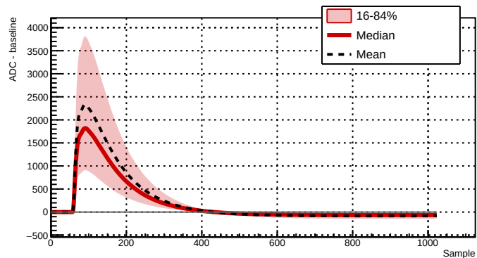
Run 039518 - Channel 2081 - 26084 waveforms
