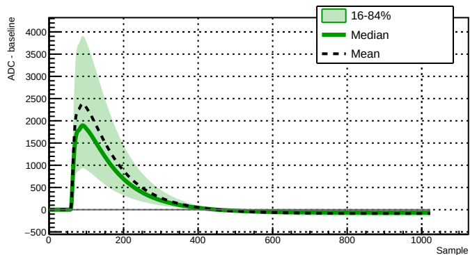
Run 039518 - Channel 2080 - 25406 waveforms
