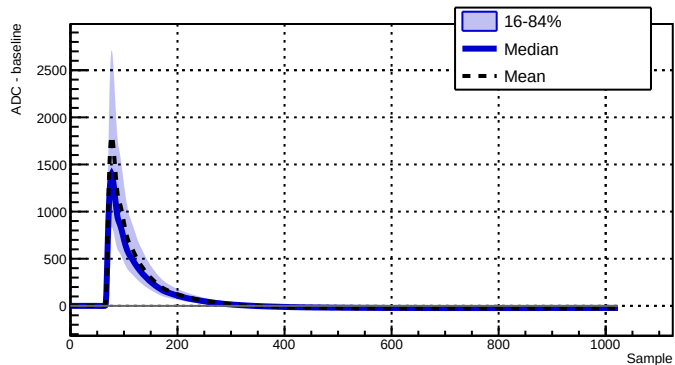
Run 039518 - Channel 2070 - 5509 waveforms
