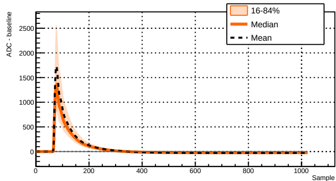
Run 039518 - Channel 2071 - 5852 waveforms
