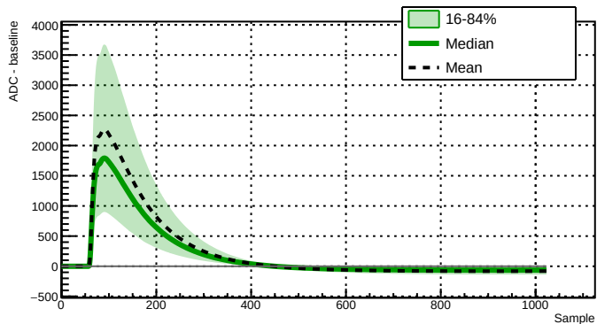
Run 039521 - Channel 2080 - 24062 waveforms
