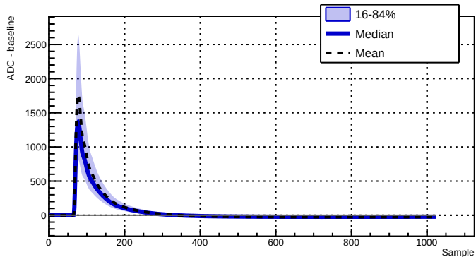
Run 039521 - Channel 2070 - 5251 waveforms
