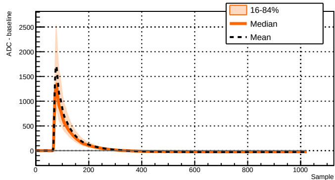
Run 039521 - Channel 2071 - 5564 waveforms
