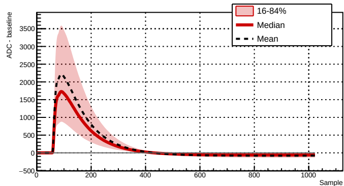
Run 039521 - Channel 2081 - 24546 waveforms
