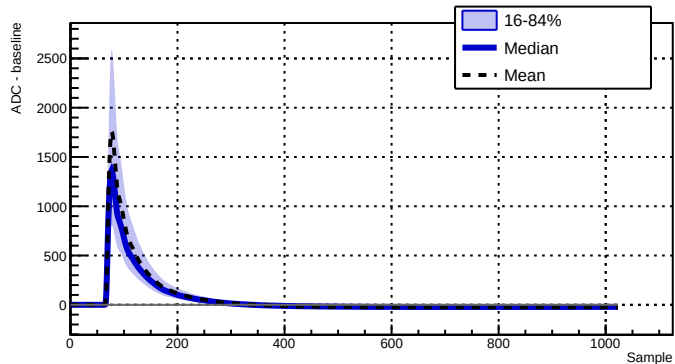
Run 039522 - Channel 2070 - 5260 waveforms
