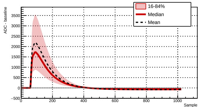
Run 039522 - Channel 2081 - 24486 waveforms
