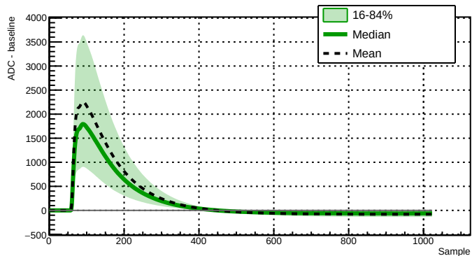
Run 039522 - Channel 2080 - 23760 waveforms
