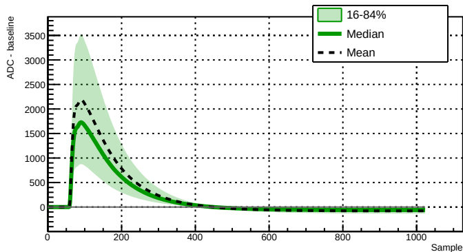
Run 039523 - Channel 2080 - 23064 waveforms
