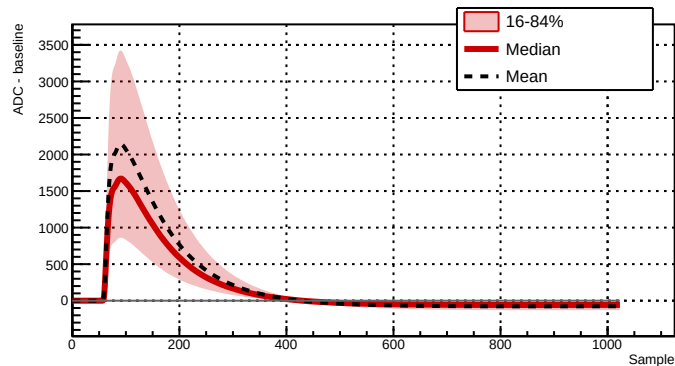
Run 039523 - Channel 2081 - 23697 waveforms
