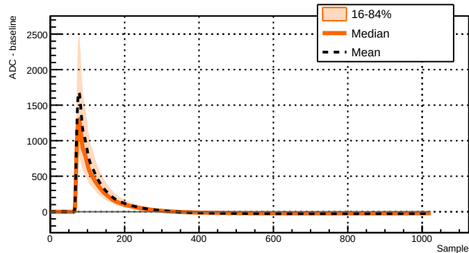
Run 039523 - Channel 2071 - 5252 waveforms
