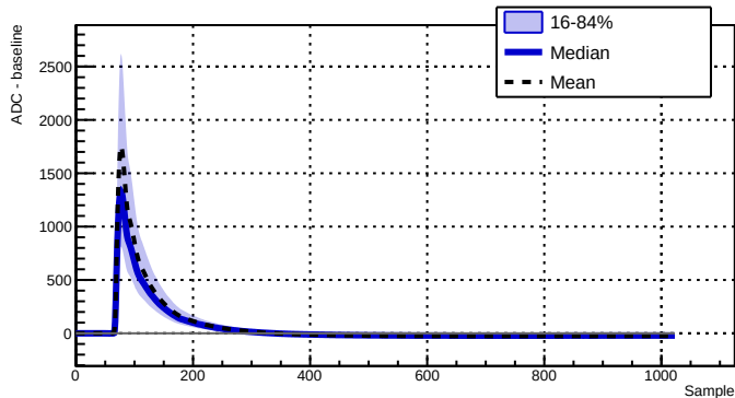
Run 039523 - Channel 2070 - 5010 waveforms
