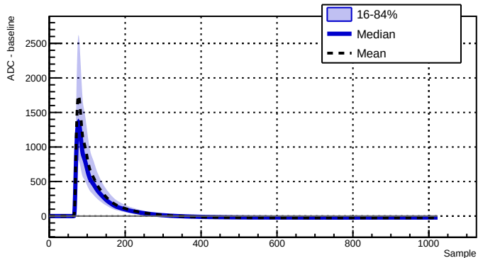
Run 039526 - Channel 2070 - 4916 waveforms
