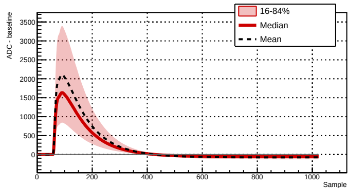
Run 039526 - Channel 2081 - 22834 waveforms
