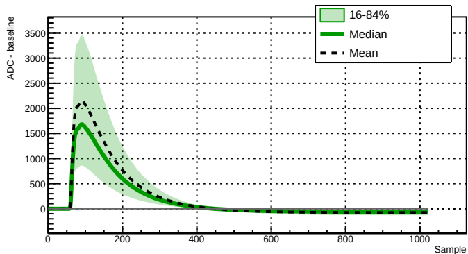
Run 039526 - Channel 2080 - 22292 waveforms
