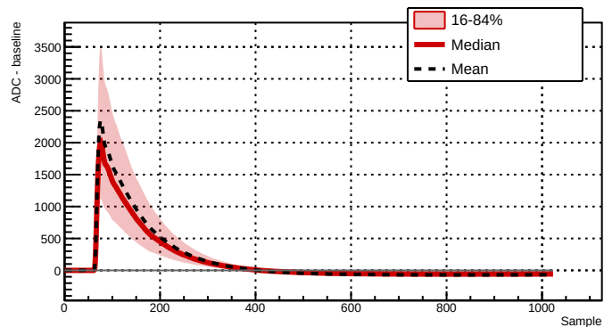
Run 039500 - Channel 2061 - 3562 waveforms
