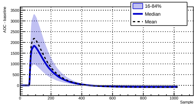
Run 039500 - Channel 2050 - 7977 waveforms
