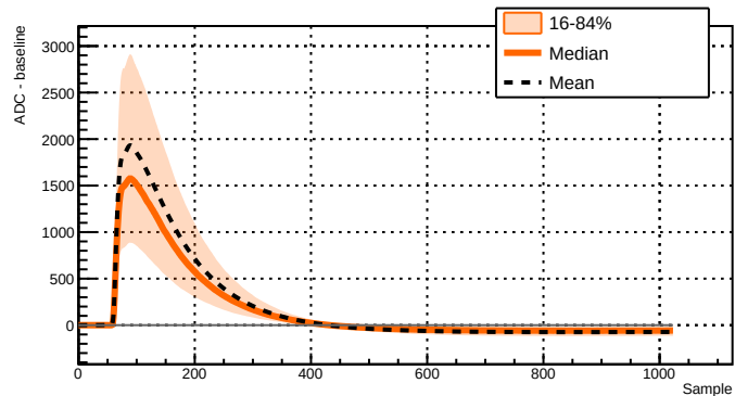
Run 039500 - Channel 2051 - 5543 waveforms
