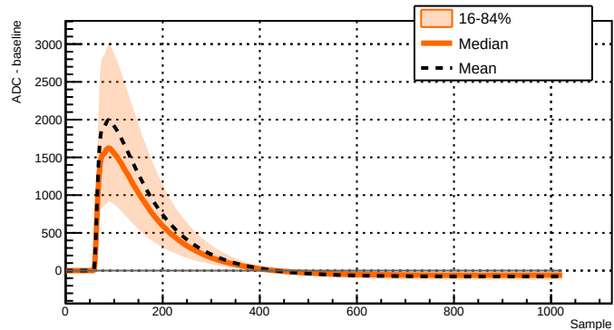
Run 039501 - Channel 2051 - 5988 waveforms
