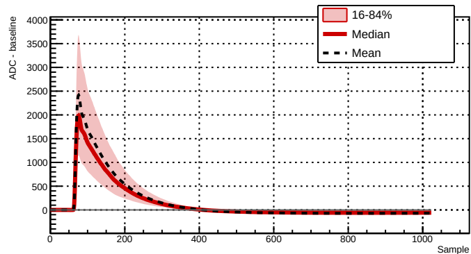
Run 039501 - Channel 2061 - 3869 waveforms
