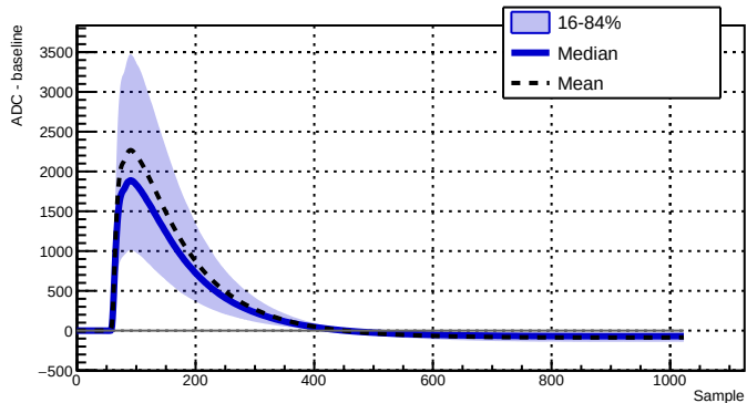
Run 039501 - Channel 2050 - 8398 waveforms
