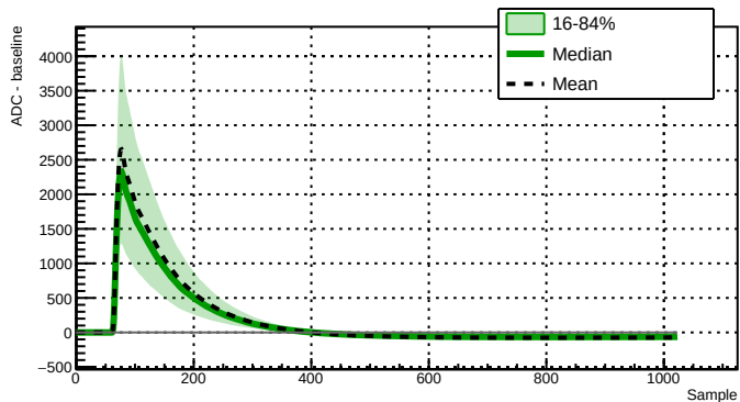
Run 039501 - Channel 2060 - 5754 waveforms
