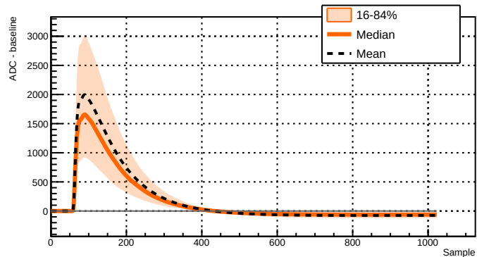
Run 039502 - Channel 2051 - 6298 waveforms
