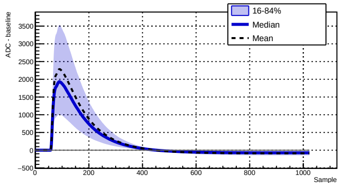
Run 039502 - Channel 2050 - 8800 waveforms
