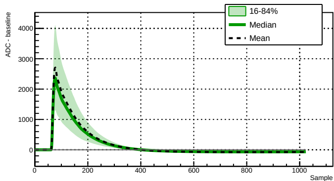
Run 039502 - Channel 2060 - 6233 waveforms
