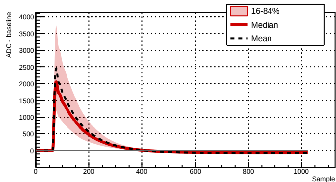
Run 039502 - Channel 2061 - 3989 waveforms
