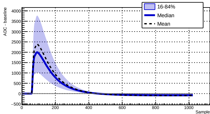
Run 039503 - Channel 2050 - 9477 waveforms
