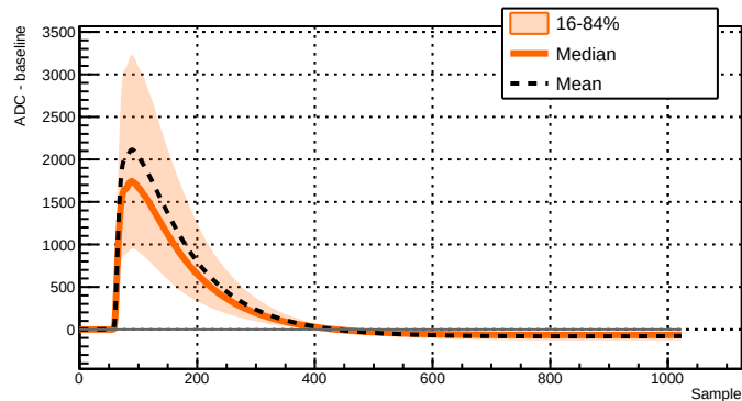
Run 039503 - Channel 2051 - 6659 waveforms
