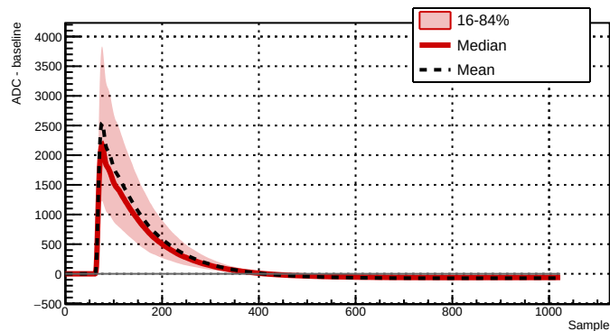
Run 039503 - Channel 2061 - 4425 waveforms
