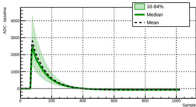
Run 039503 - Channel 2060 - 6690 waveforms
