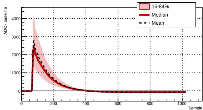
Run 039506 - Channel 2061 - 5534 waveforms
