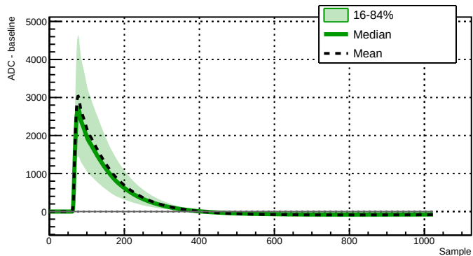
Run 039506 - Channel 2060 - 7906 waveforms
