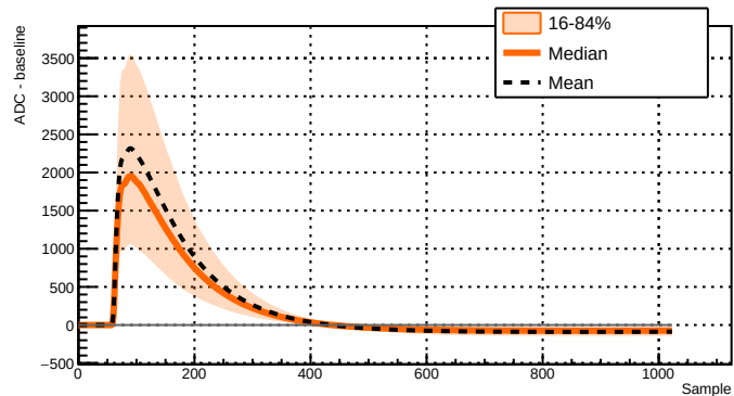
Run 039506 - Channel 2051 - 7980 waveforms
