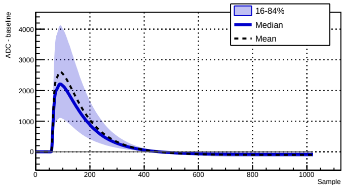
Run 039506 - Channel 2050 - 10989 waveforms
