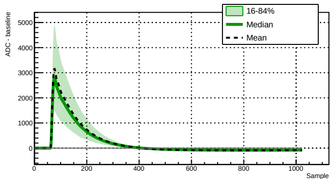
Run 039507 - Channel 2060 - 8847 waveforms
