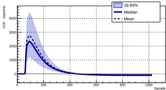
Run 039507 - Channel 2050 - 12040 waveforms
