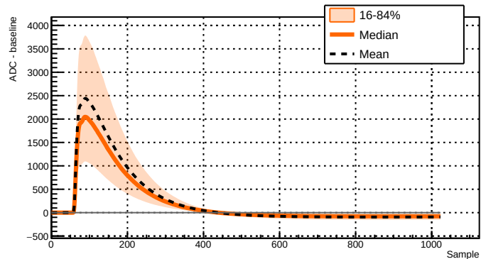
Run 039507 - Channel 2051 - 8901 waveforms
