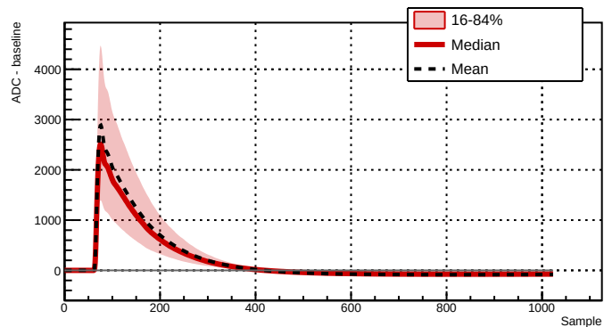
Run 039507 - Channel 2061 - 6076 waveforms
