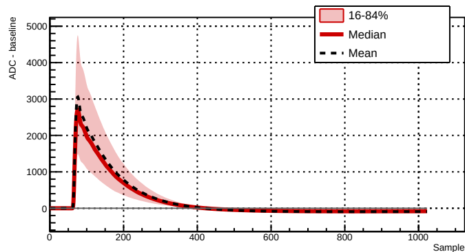
Run 039508 - Channel 2061 - 6626 waveforms
