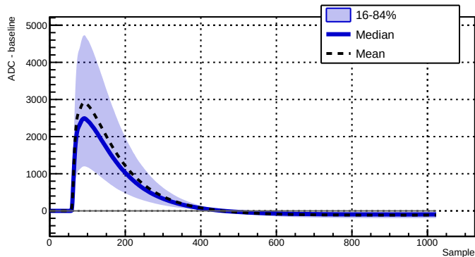
Run 039508 - Channel 2050 - 12825 waveforms
