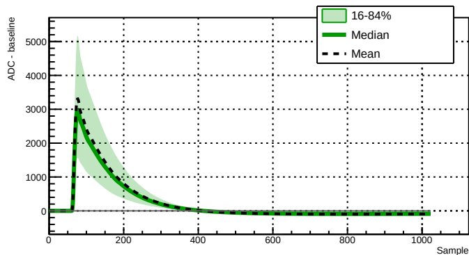
Run 039508 - Channel 2060 - 9388 waveforms
