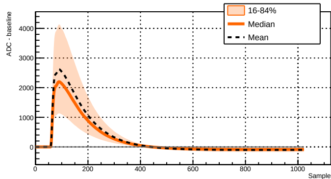
Run 039508 - Channel 2051 - 9676 waveforms
