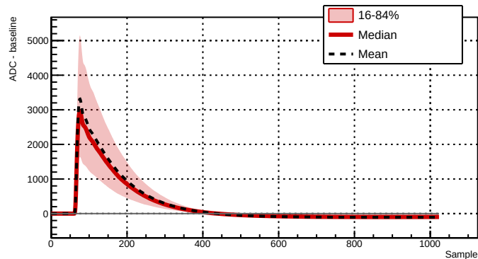
Run 039510 - Channel 2061 - 6744 waveforms
