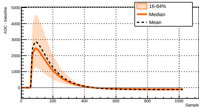
Run 039510 - Channel 2051 - 10437 waveforms
