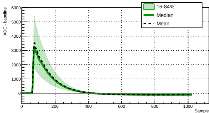
Run 039510 - Channel 2060 - 9797 waveforms
