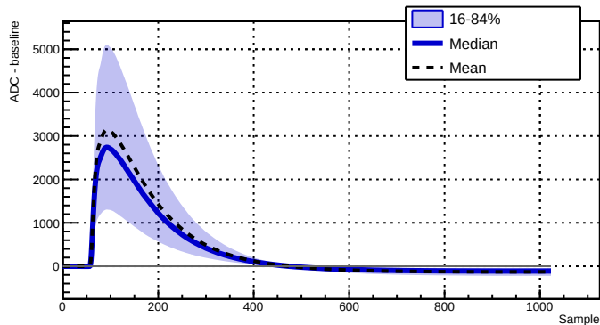
Run 039510 - Channel 2050 - 13465 waveforms
