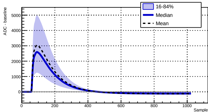
Run 039511 - Channel 2050 - 13722 waveforms
