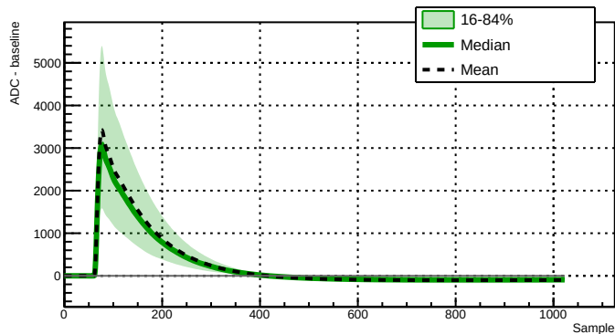
Run 039511 - Channel 2060 - 10165 waveforms
