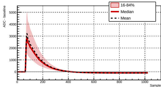
Run 039511 - Channel 2061 - 7134 waveforms
