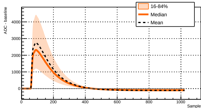
Run 039511 - Channel 2051 - 10541 waveforms
