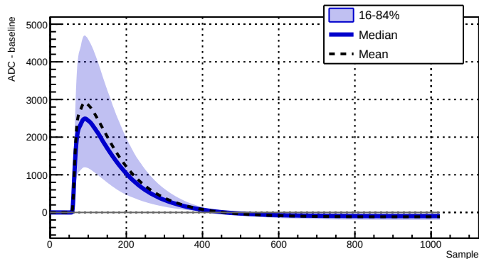
Run 039512 - Channel 2050 - 13048 waveforms
