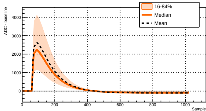
Run 039512 - Channel 2051 - 9968 waveforms
