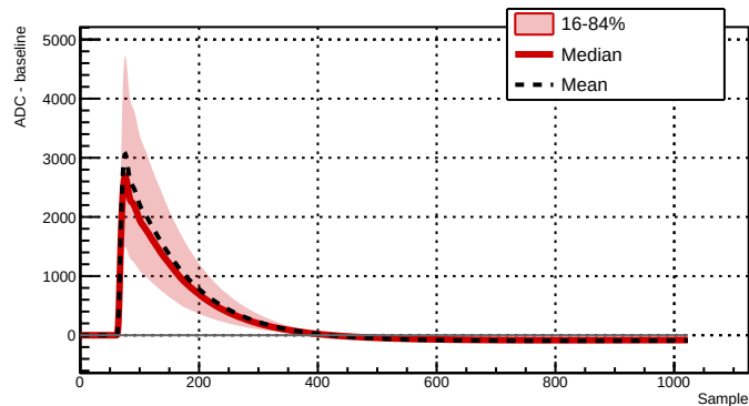
Run 039512 - Channel 2061 - 6862 waveforms
