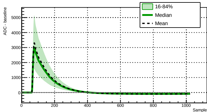
Run 039512 - Channel 2060 - 9660 waveforms
