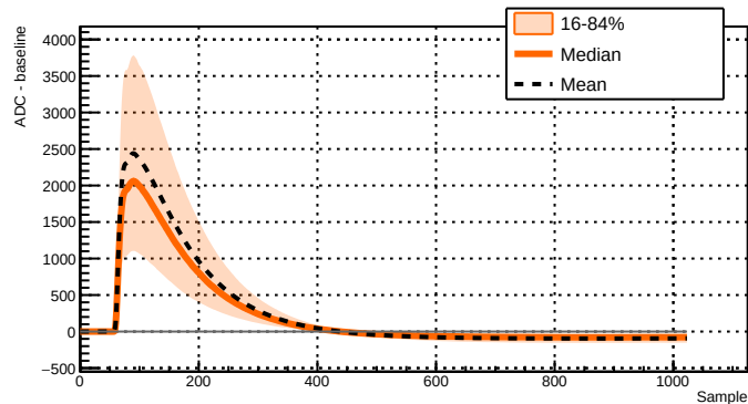
Run 039515 - Channel 2051 - 8703 waveforms
