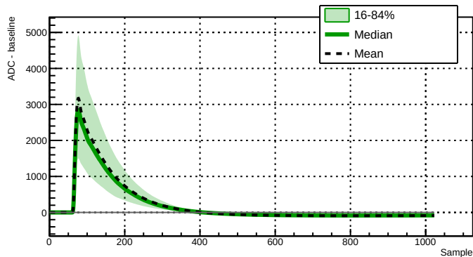
Run 039515 - Channel 2060 - 8566 waveforms
