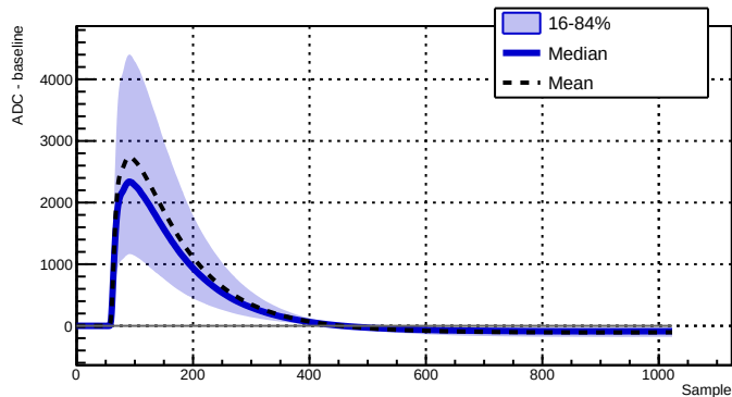
Run 039515 - Channel 2050 - 11682 waveforms
