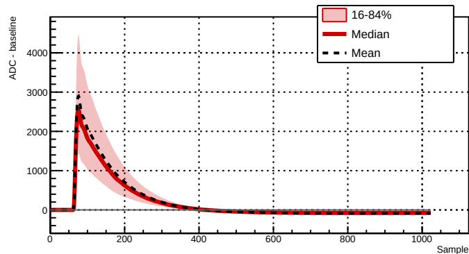
Run 039515 - Channel 2061 - 5887 waveforms
