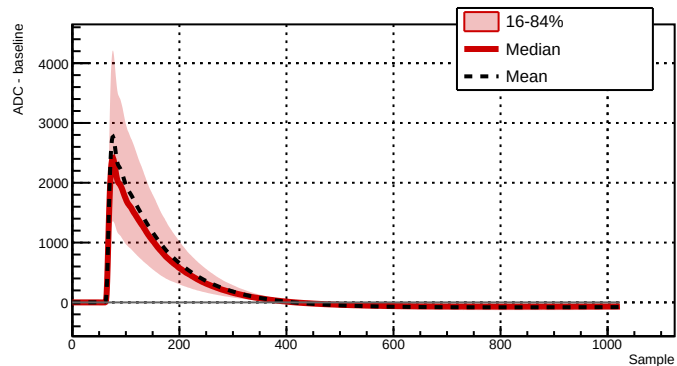
Run 039517 - Channel 2061 - 5397 waveforms
