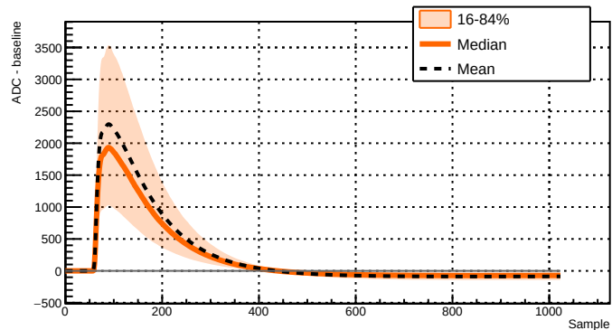
Run 039517 - Channel 2051 - 8065 waveforms
