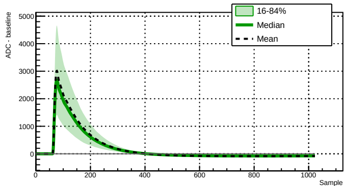
Run 039517 - Channel 2060 - 8050 waveforms
