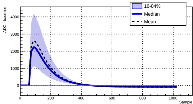
Run 039517 - Channel 2050 - 11046 waveforms
