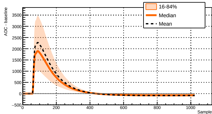
Run 039518 - Channel 2051 - 7596 waveforms
