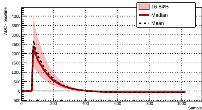
Run 039518 - Channel 2061 - 5085 waveforms
