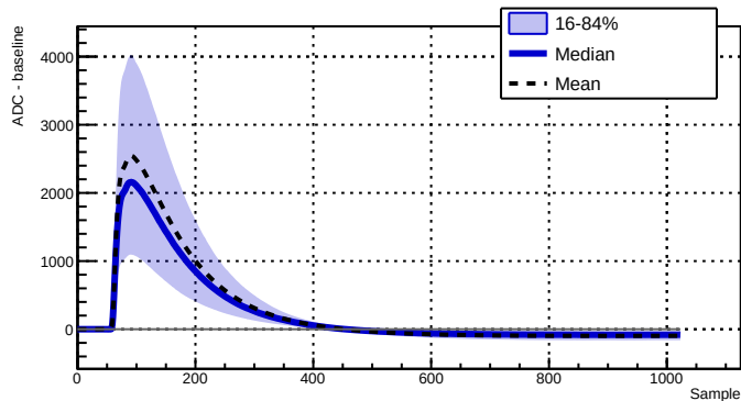
Run 039518 - Channel 2050 - 10502 waveforms
