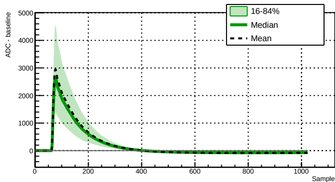
Run 039518 - Channel 2060 - 7585 waveforms
