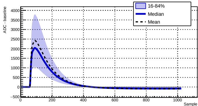
Run 039521 - Channel 2050 - 9769 waveforms
