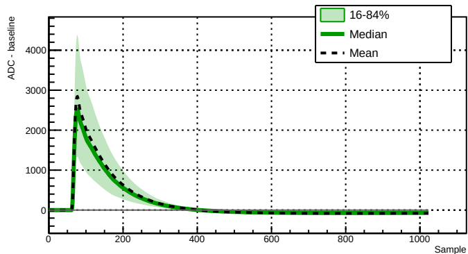
Run 039521 - Channel 2060 - 7007 waveforms
