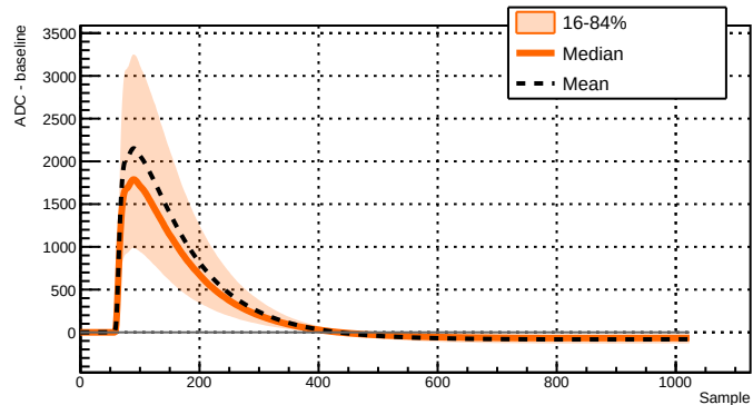
Run 039521 - Channel 2051 - 6981 waveforms
