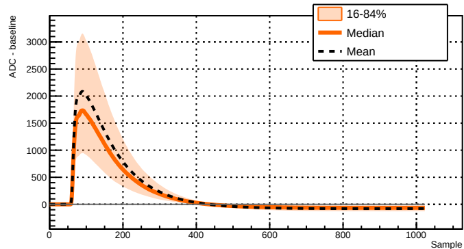
Run 039522 - Channel 2051 - 6764 waveforms
