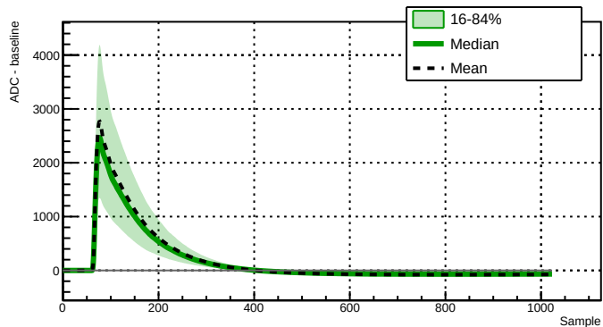
Run 039522 - Channel 2060 - 6650 waveforms
