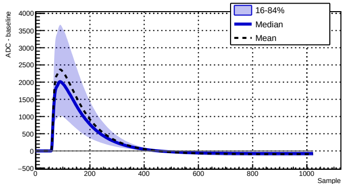
Run 039522 - Channel 2050 - 9398 waveforms
