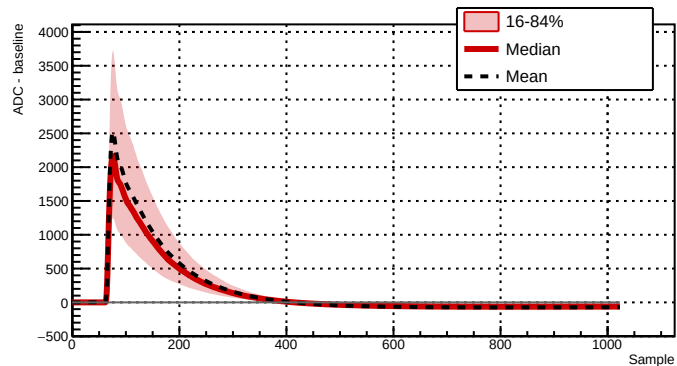
Run 039522 - Channel 2061 - 4434 waveforms
