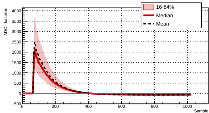
Run 039523 - Channel 2061 - 4420 waveforms
