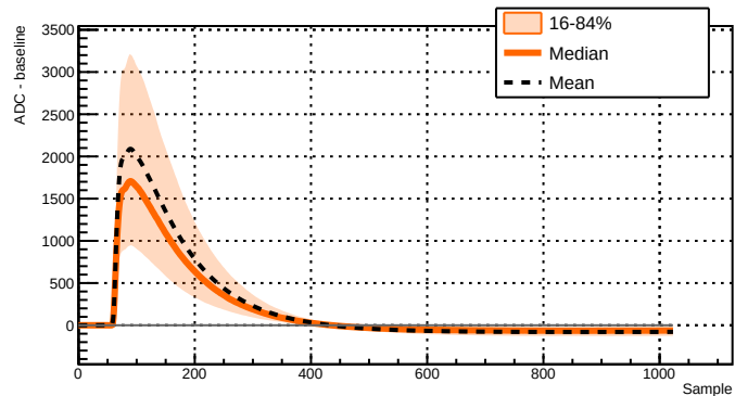
Run 039523 - Channel 2051 - 6424 waveforms
