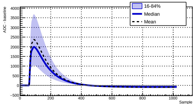
Run 039523 - Channel 2050 - 9164 waveforms
