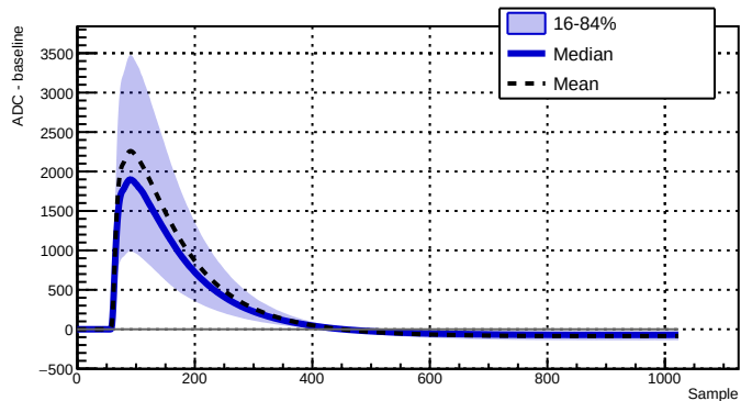
Run 039526 - Channel 2050 - 8743 waveforms
