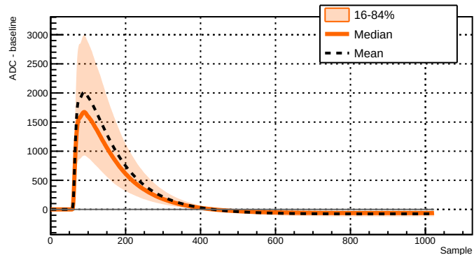
Run 039526 - Channel 2051 - 6014 waveforms
