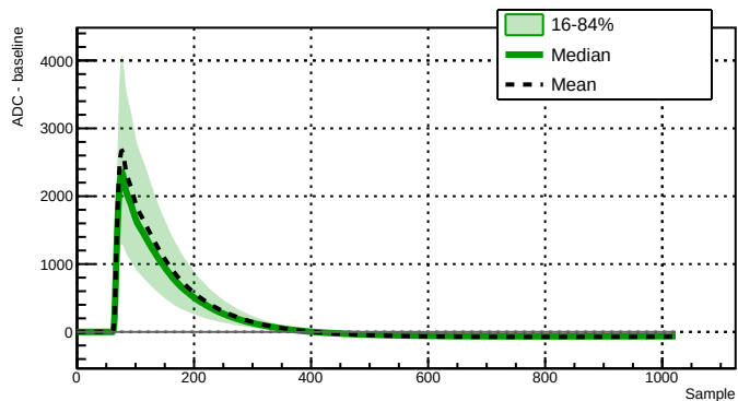
Run 039526 - Channel 2060 - 6008 waveforms
