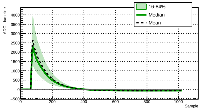
Run 039527 - Channel 2060 - 5832 waveforms
