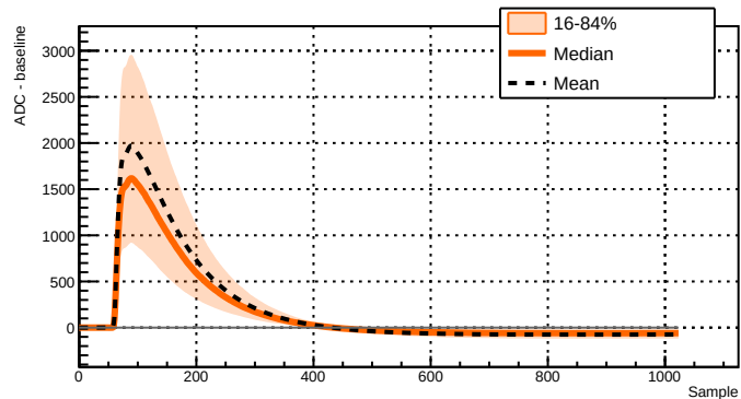
Run 039527 - Channel 2051 - 5866 waveforms
