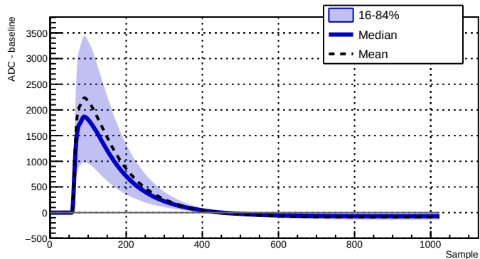
Run 039527 - Channel 2050 - 8474 waveforms
