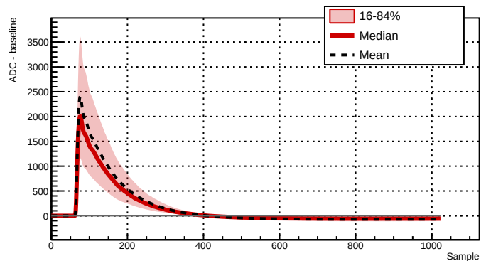
Run 039527 - Channel 2061 - 3814 waveforms
